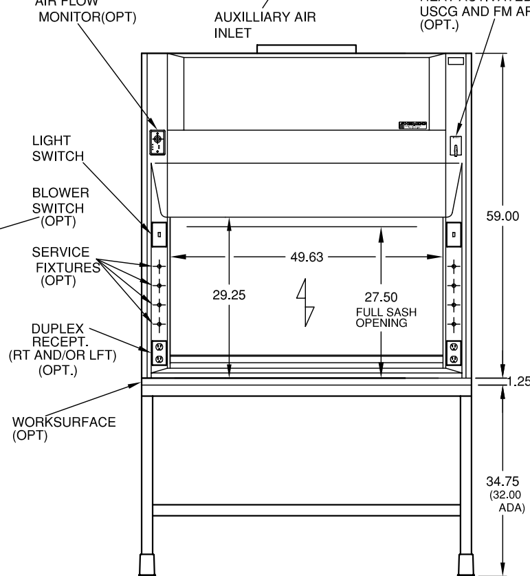
CAT. NO. 21521 (WITH OPTIONAL TABLE AND WORKSURFACE)
