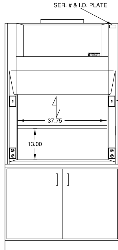
CAT. NO. 21421 (WITH OPTIONAL BASE CABINET AND WORKSURFACE)
