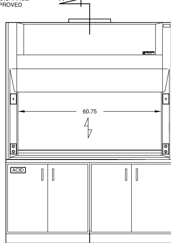
CAT. NO. 21621 (WITH OPTIONAL ACID/BASE CABINETS AND WORKSURFACE)
