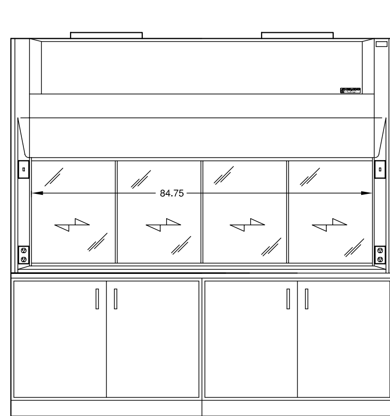
CAT. NO. 21821 (WITH OPTIONAL HORIZONTAL SLIDING SASH, BASE CABINETS AND WORKSURFACE)
