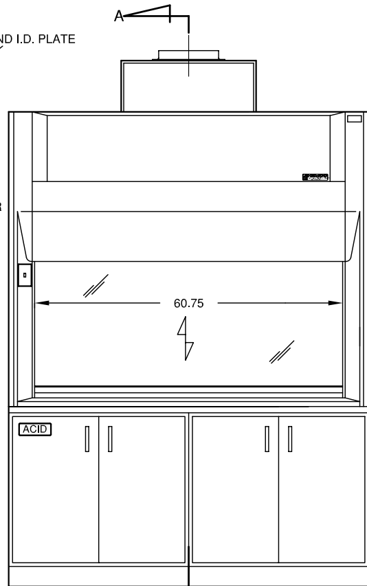
CAT. NO. 17061 (WITH OPTIONAL ACID/BASE CABINETS AND WORKSURFACE)
