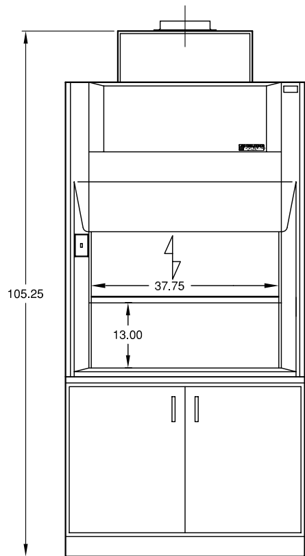
CAT. NO. 17041 (WITH OPTIONAL BASE CABINET AND WORKSURFACE)
