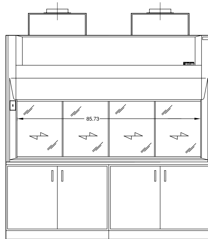
CAT. NO. 17081 (WITH OPTIONAL BASE CABINETS HORIZONTAL SLIDING SASH AND WORKSURFACE)
