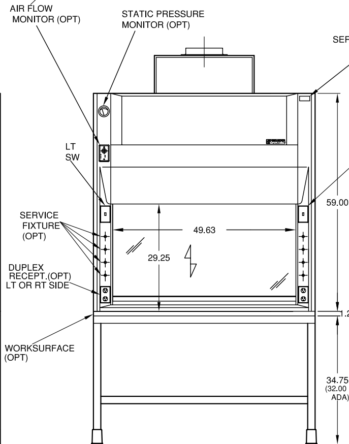
CAT. NO. 17051 (WITH OPTIONAL TABLE, WORKSURFACE, AND FULL SERVICES.)
