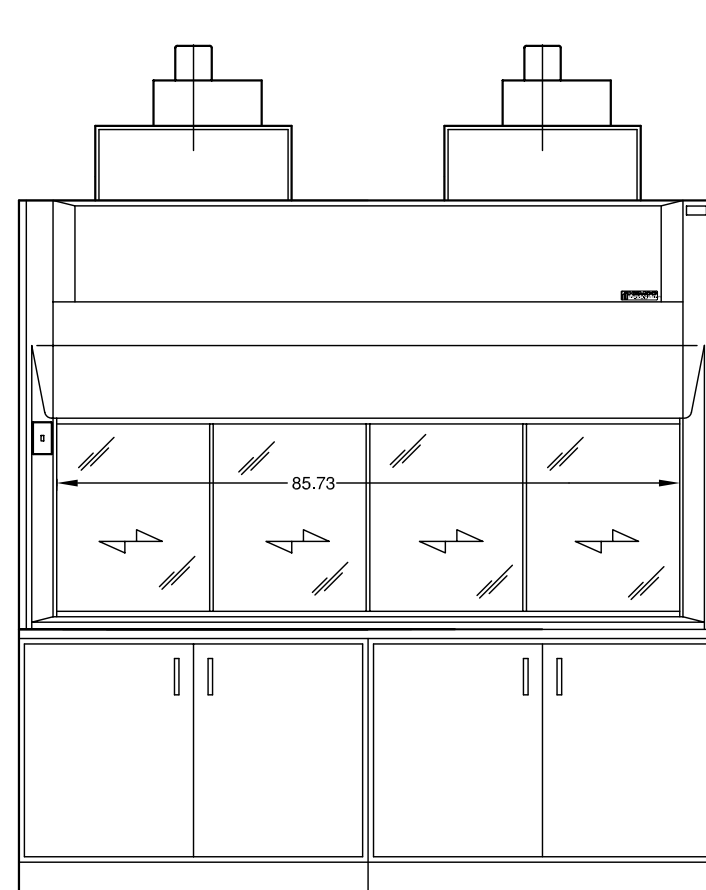
CAT. NO. 17082 (WITH OPTIONAL BASE CABINETS HORIZONTAL SLIDING SASH AND WORKSURFACE)
