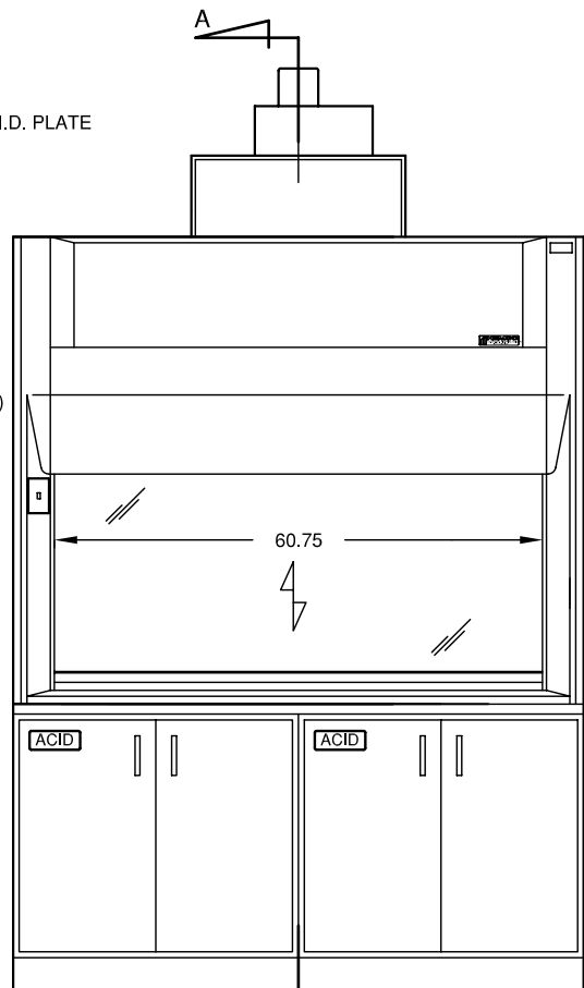
CAT. NO. 17062 (WITH OPTIONAL ACID/BASE CABINETS AND WORKSURFACE)
