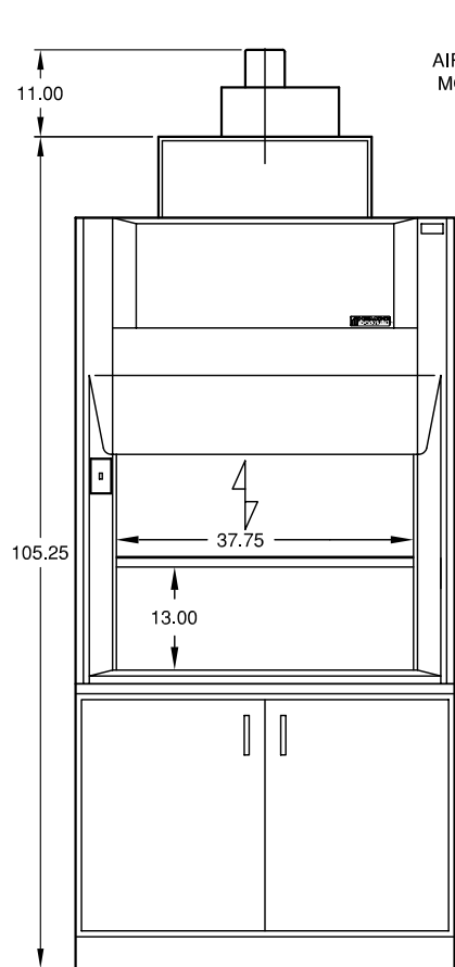
CAT. NO. 17042 (WITH OPTIONAL BASE CABINET AND WORKSURFACE)
