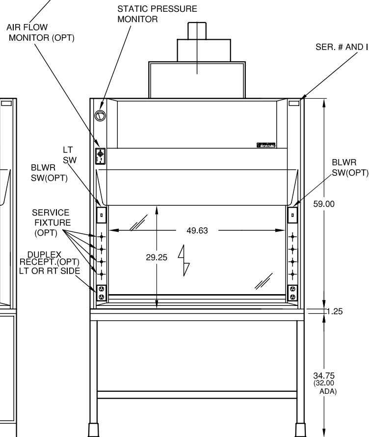
CAT. NO. 17052 (WITH OPTIONAL TABLE, WORKSURFACE AND FULL SERVICES)
