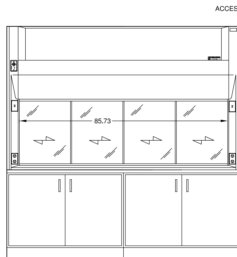
MODEL 21801 (WITH OPTIONAL HORIZONTAL SLIDING SASH, BASE CABINETS AND WORKSURFACE)
