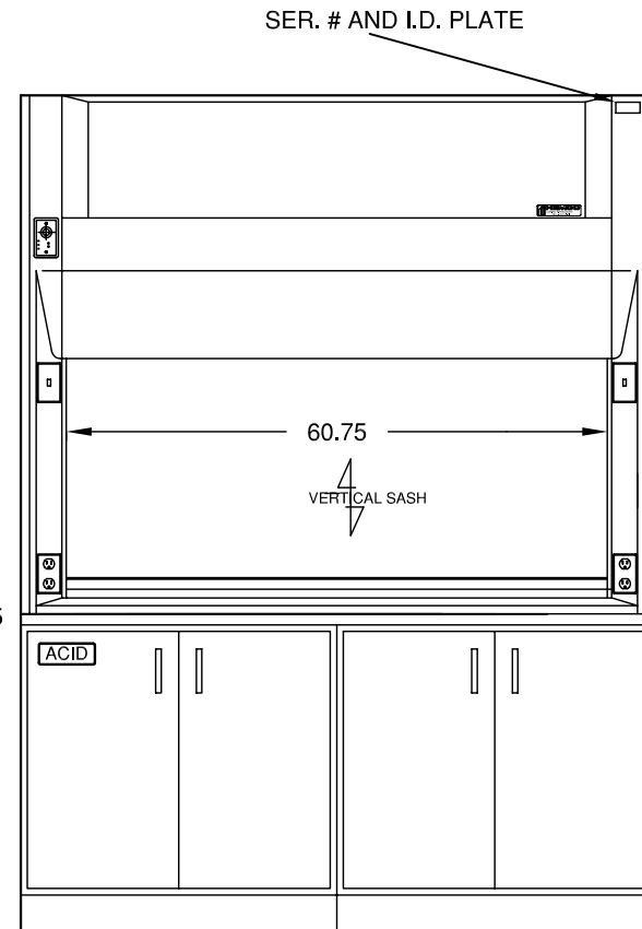
MODEL 21601 (WITH OPTIONAL ACID/BASE CABINET AND WORKSURFACE)
