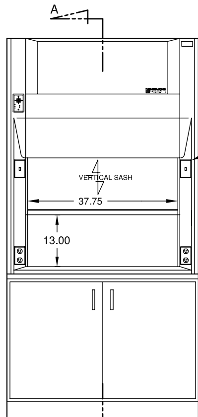
MODEL 21401 (WITH OPTIONAL BASE CABINET AND WORKSURFACE)
