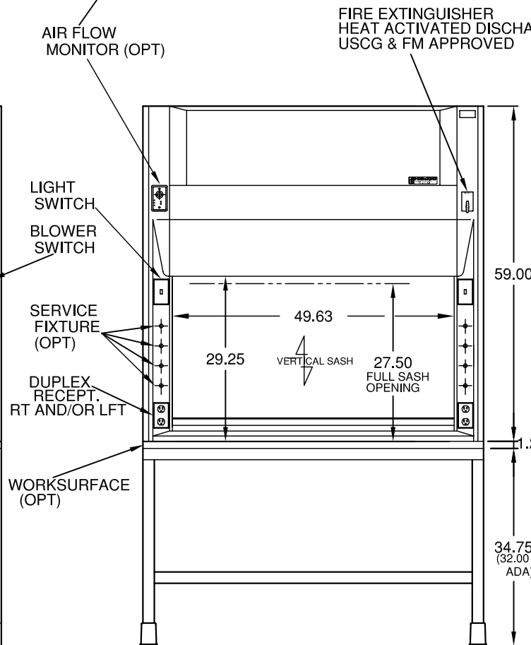
MODEL 21501 (WITH OPTIONAL TABLE AND WORKSURFACE)
