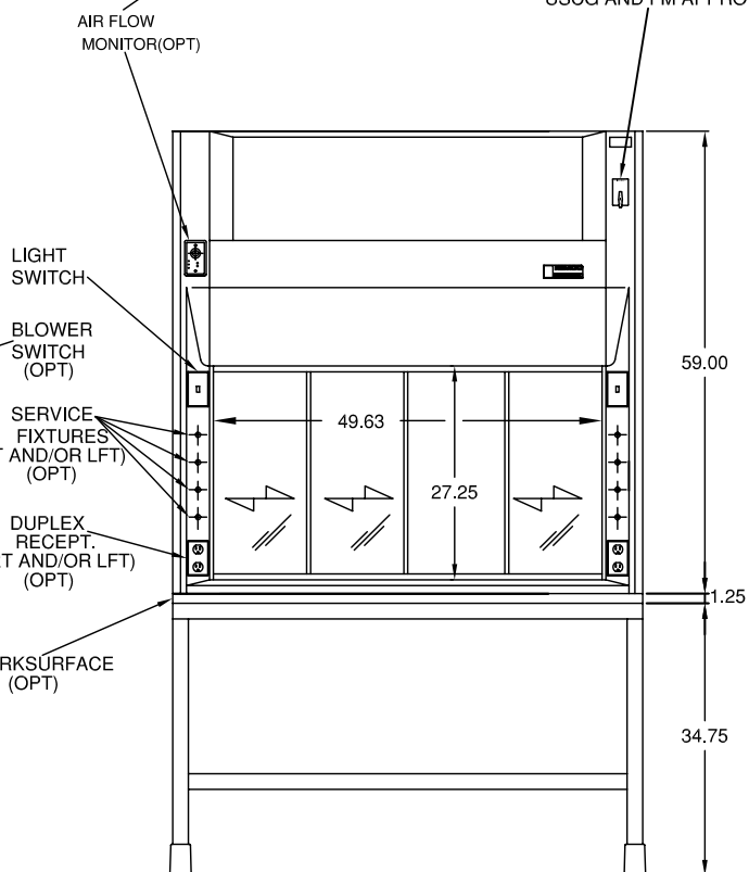
MODEL 12250 (WITH OPTIONAL TABLE AND WORKSURFACE)
