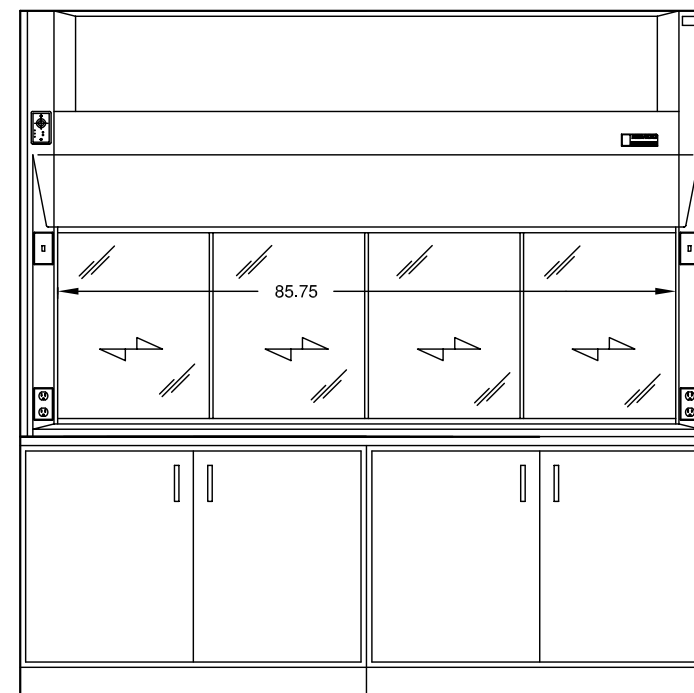
MODEL 12280 (WITH OPTIONAL BASE CABINETS AND WORKSURFACE)
