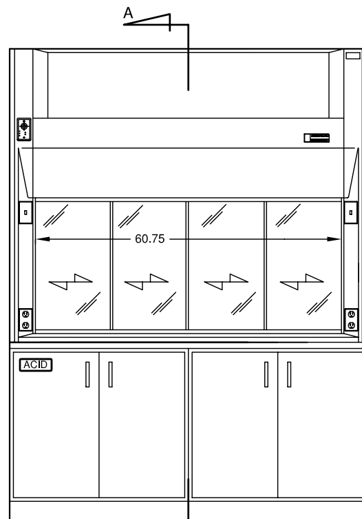
MODEL 12260 (WITH OPTIONAL ACID/BASE CABINETS AND WORKSURFACE)
