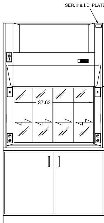
MODEL 12240 (WITH OPTIONAL BASE CABINET AND WORKSURFACE)
