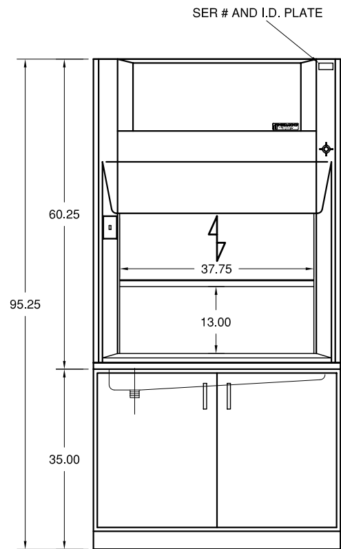
CAT. NO. 13411 (WITH OPTIONAL BASE CABINET)
