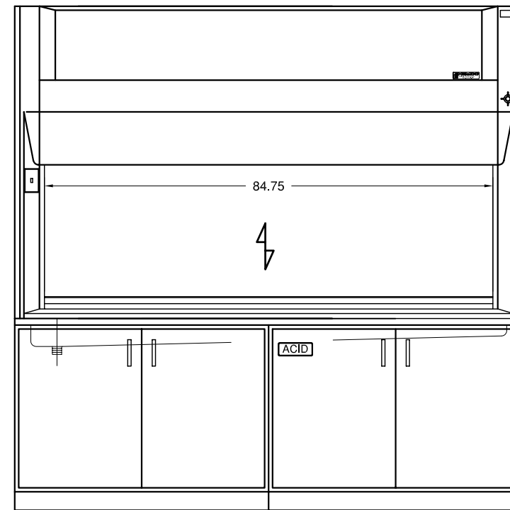
CAT. NO. 13811 (WITH OPTIONAL BASE CABINET)
