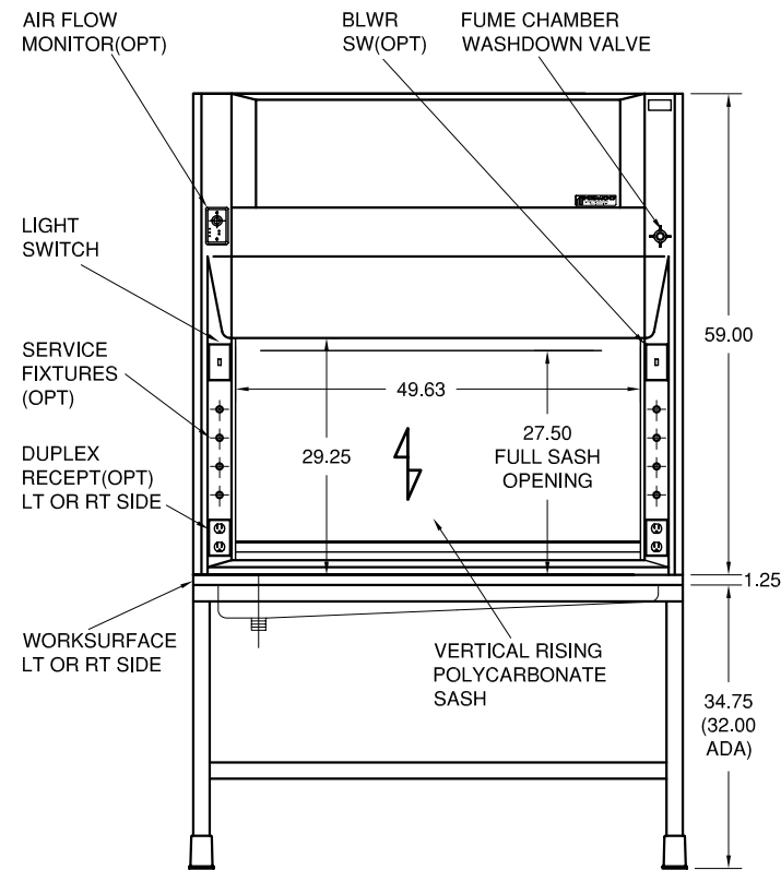
CAT. NO. 13511 (WITH OPTIONAL TABLE)
