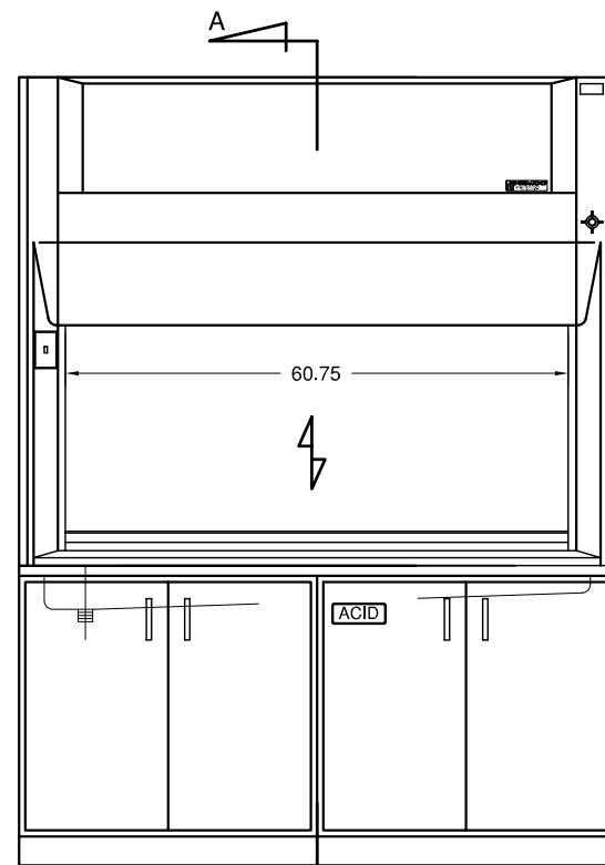
CAT. NO. 13611 (WITH OPTIONAL ACID/BASE CABINETS)
