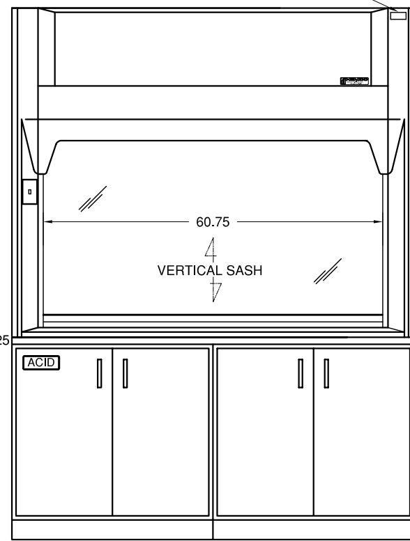
CAT. NO. 45611 (WITH OPTIONAL ACID/BASE CABINETS AND WORKSURFACE)
