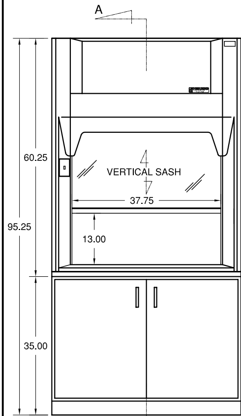
CAT. NO. 45411 (WITH OPTIONAL BASE CABINET AND WORKSURFACE)
