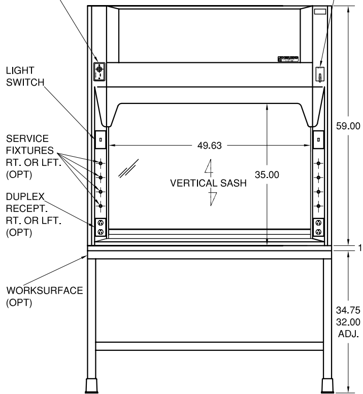
CAT. NO. 45511 (WITH OPTIONAL TABLE AND WORKSURFACE)
