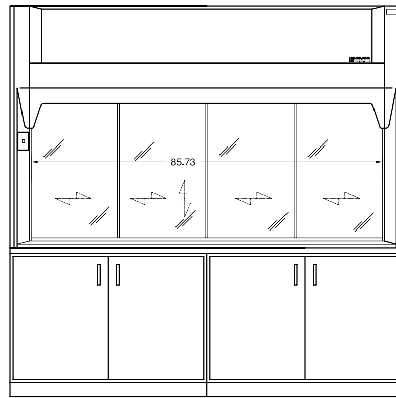
CAT. NO. 45811 (WITH OPTIONAL HORIZONTAL SLIDING SASH AND BASE CABINETS AND WORKSURFACE)
