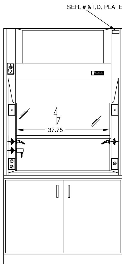
MODEL 14401 (WITH OPTIONAL BASE CABINET)
