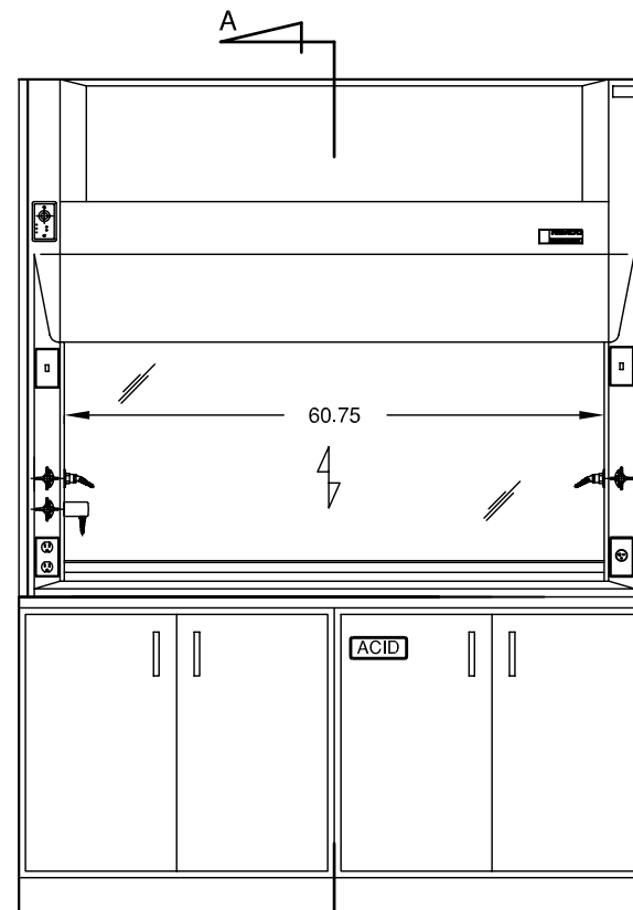
MODEL 14601 (WITH OPTIONAL ACID/BASE CABINETS)
