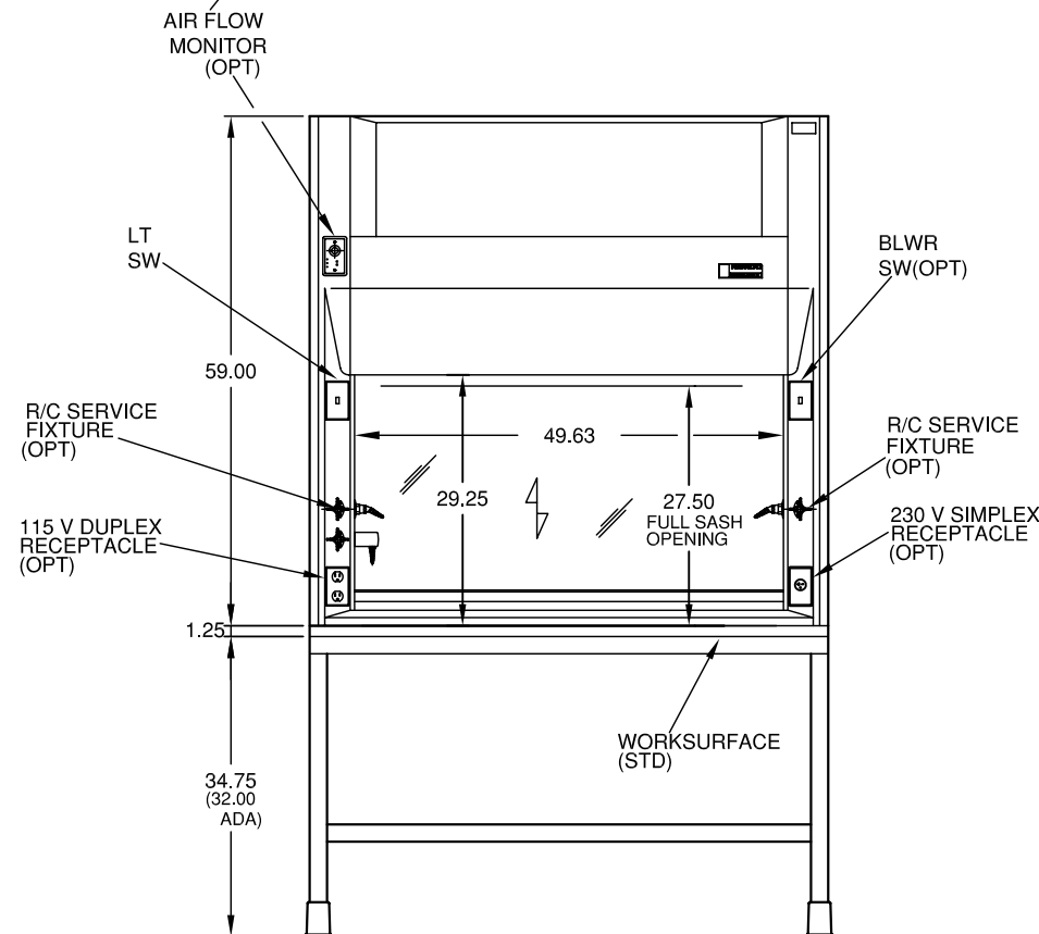
MODEL 14501 (WITH OPTIONAL TABLE)
